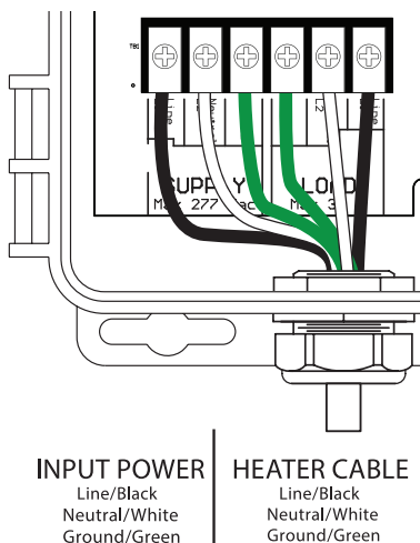
FIGURE 3.2 Contactor Connections
